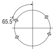
Coolant Inlet Port 8WCB (4) 0.531 (13,5)Ø Dia. Mounting holes based on 6 equally spaced as shown on 11.125 (282,5) bolt circle
