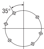
Coolant Inlet Port 14WCB (6) 0.656 (16,7)Ø Dia. Mounting holes based on 8 equally spaced as shown on 17.500 (444,5) bolt circle
